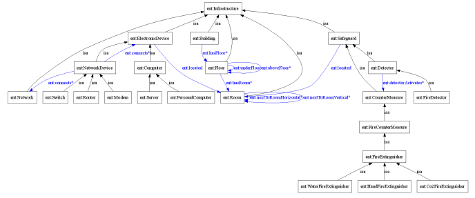
Fig. 3. Sub-tree 'ent:Infrastructure'
