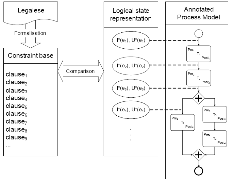
Fig. 6 An overview of the framework [34]
