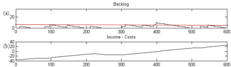
Fig. 15 Simulation result excerpt: silver level
