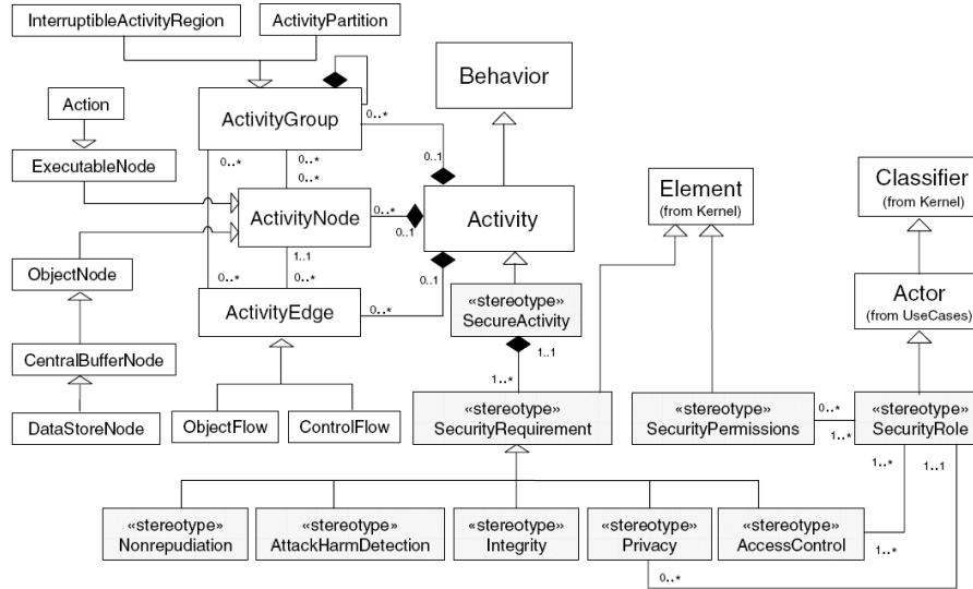
Fig. 3 Extending the UML 2.0 meta-model with security stereotypes [27]
