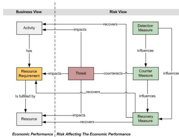
Fig. 12 Reference Model applied on the Business Process Elements Activity, Resource Requirement and Resource [18]
