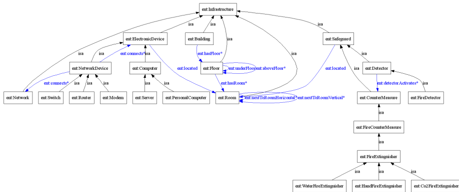
Fig. 3. Sub-tree 'ent:Infrastructure'
