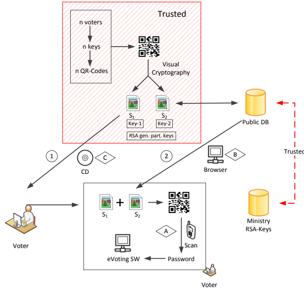
Fig. 6. Attacker model.
